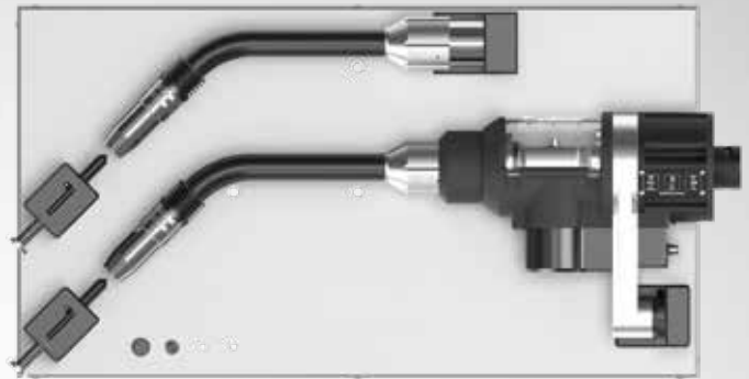
Top view checking fixture
