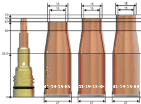
Gas nozzle PART-NO. 41-19-15-BS 41-19-15-BF 41-19-15-BR
