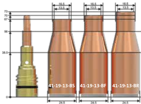
Gas nozzle PART-NO. 41-19-13-BS 41-19-13-BF 41-19-13-BR
