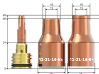
Gas nozzle PART-NO. 41-21-13-BS 41-21-13-BF
