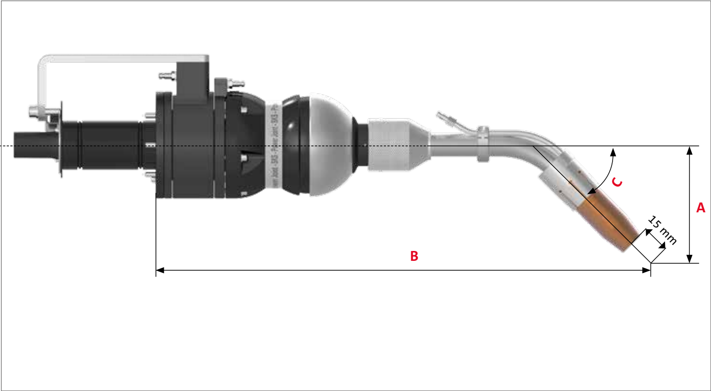
Overview of water-cooled torch necks
