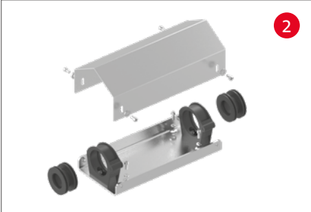
Connection bracket
